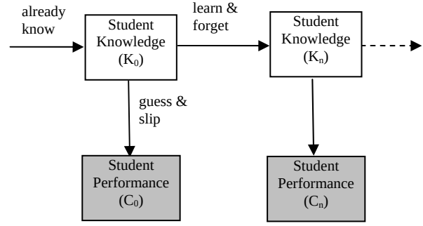
Figure 1 Graphical representation of Knowledge Tracing
