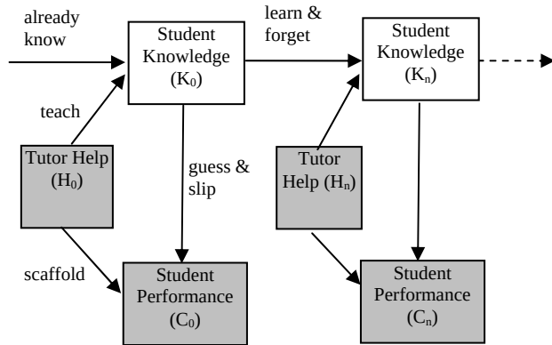
Figure 2 Graphical representation of the Help model
