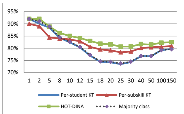
Figure 2. Accuracy on student's 1 st , 2 nd , 3 rd , ... test steps
