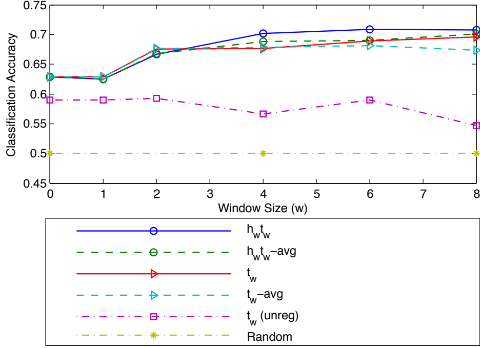
Fig. 3. Classification accuracy for Task Completion
